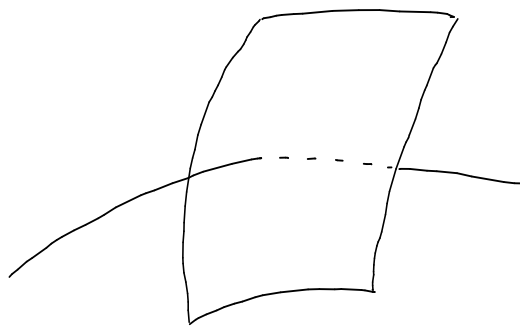
An algebraic set with two irreducible components.
