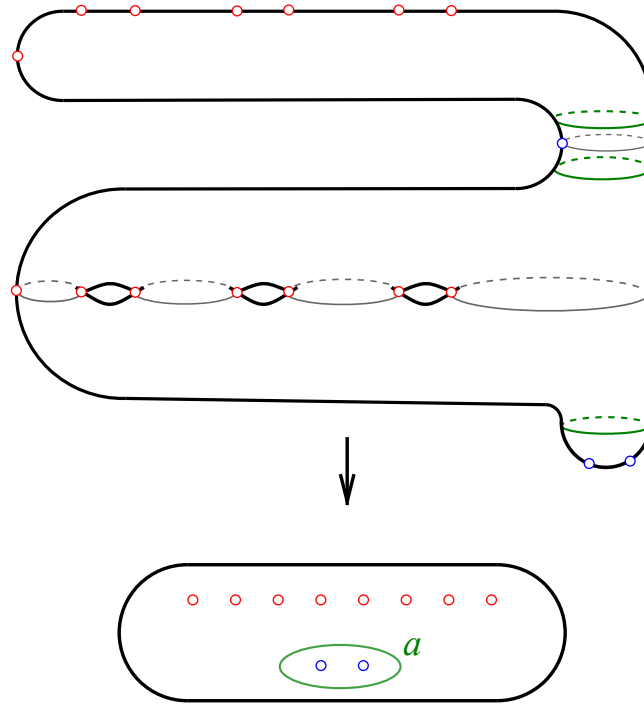
FIGURE 1. The simple threefold cover of S_g over the sphere. The gray curves divide S_g into three regions, each serving as a “fundamental domain” for the cover. The preimages in S_g of the branch points in S^2 are shown as dots but are treated as unmarked points in S_g .
