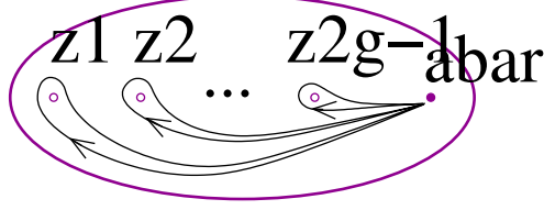
FIGURE 4. The generators x_i for \pi_1(D_{2g-1}^\circ) .
