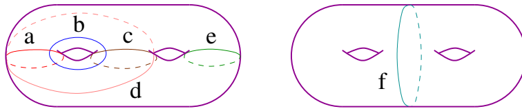
FIGURE 5. The curves a , b , c , d , e , and f from Theorem 2.1.
